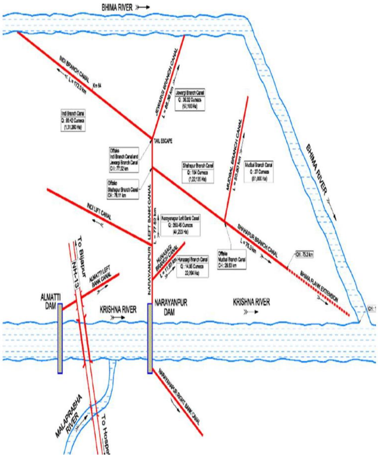
Canal Network Schematic
